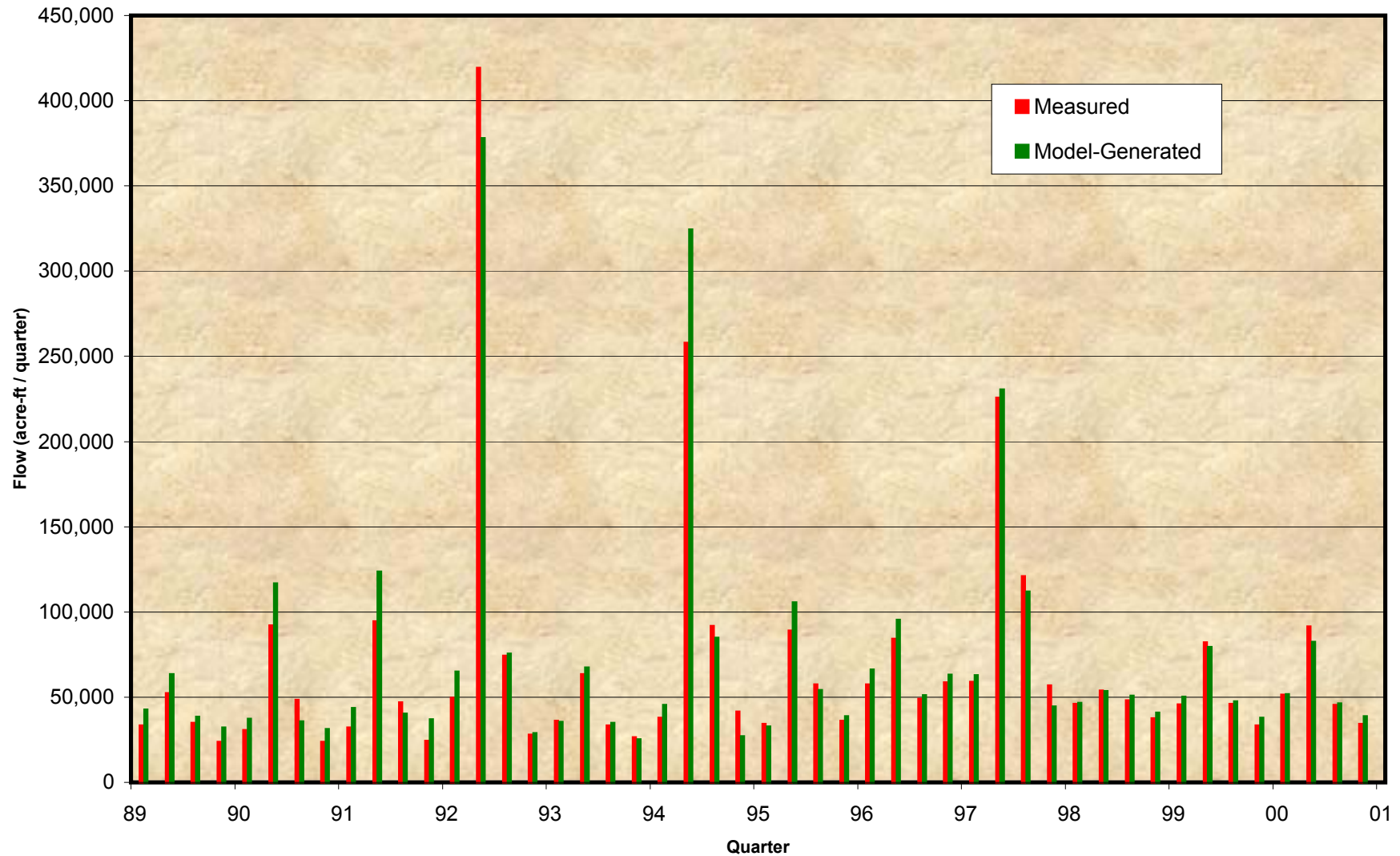
Figure 6-17a Comparison of Model-Projected and Observed Santa Ana River Discharge Time Histories at Prado Dam – Histogram
