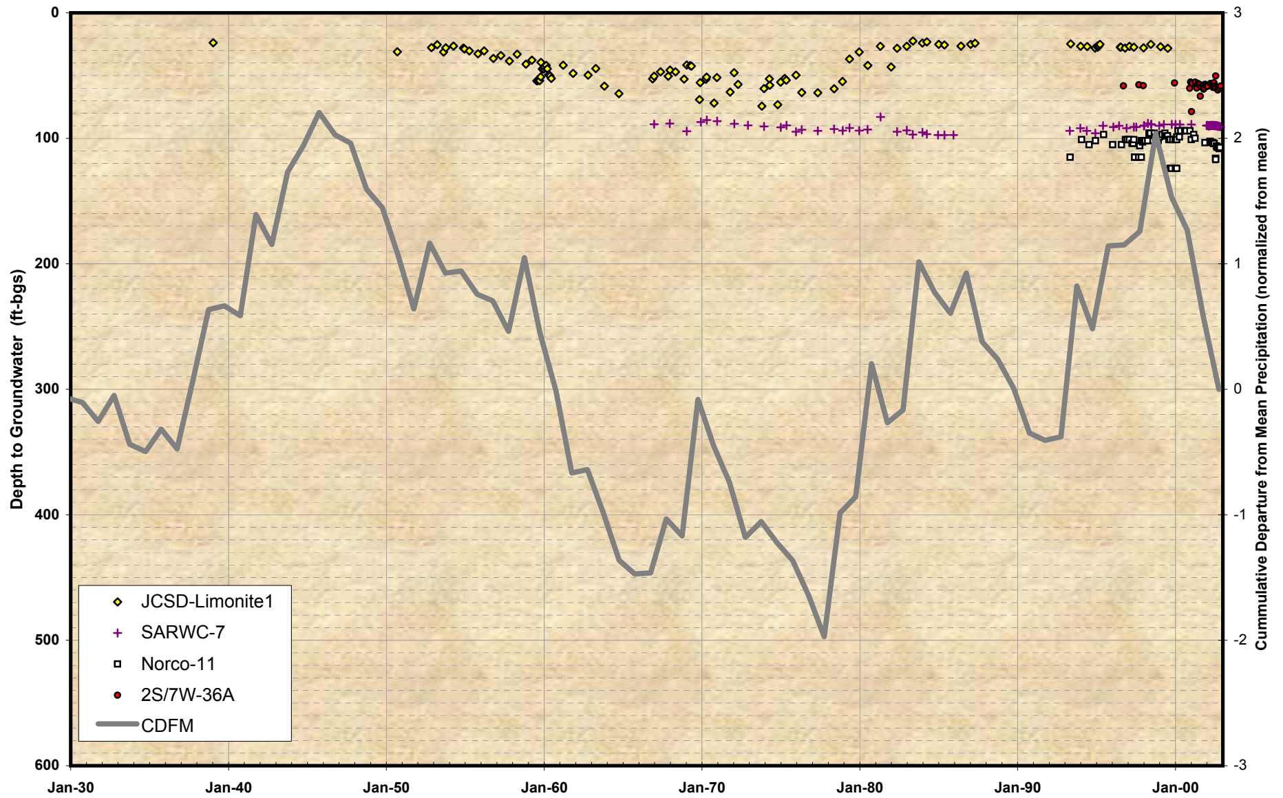
Figure 2-23 Water-Level Time Histories at Wells in Management Zone 5
