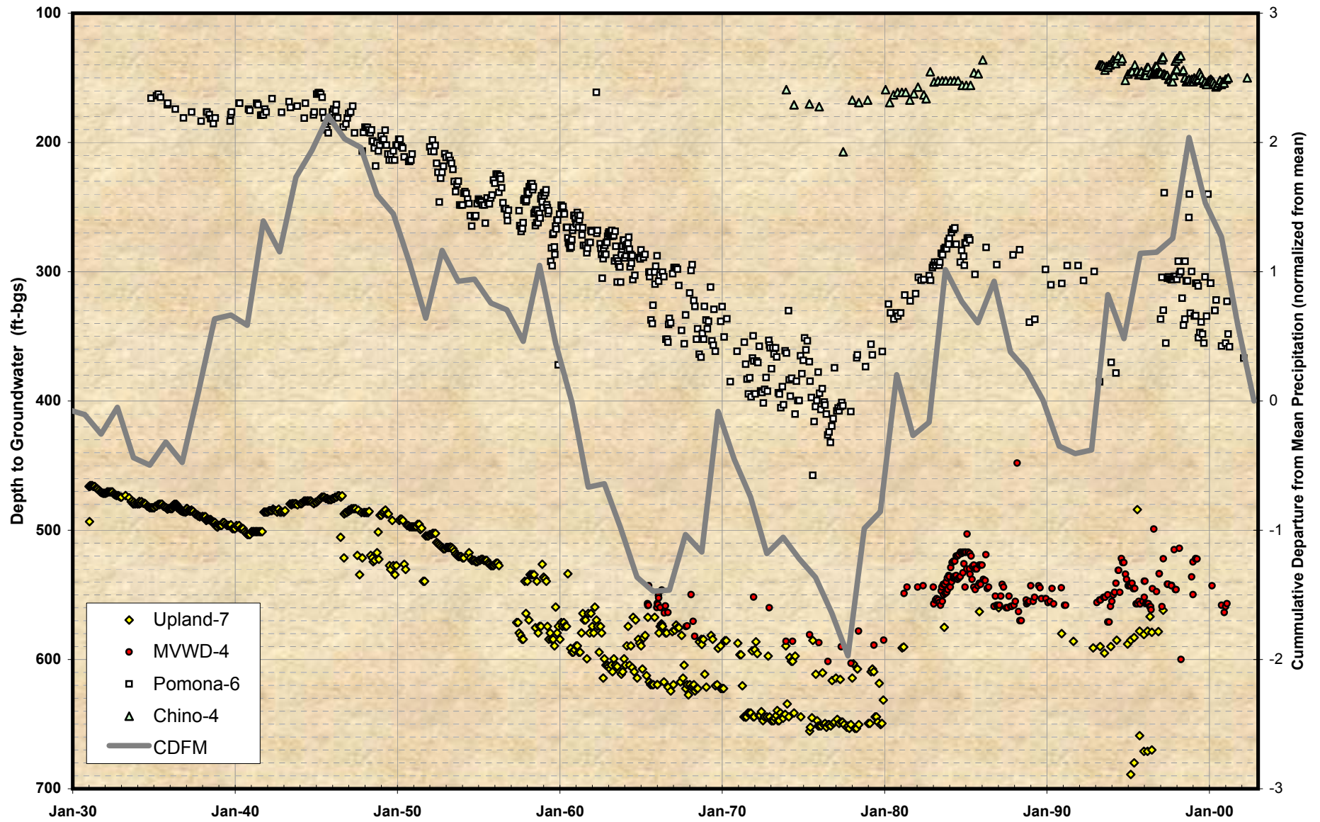
Figure 2-19 Water-Level Time Histories at Wells in Management Zone 1
