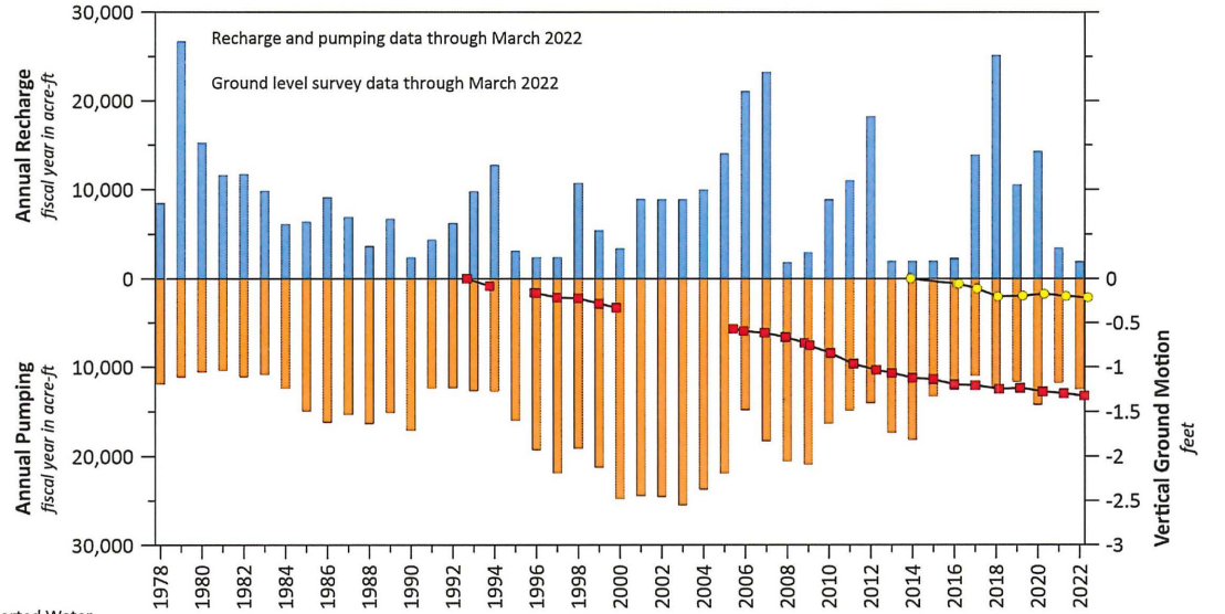
Figure 3-9 History of Land Subsidence in Northwest MZ-1 Ground-Level Monitoring Committee 2021/22 Annual Report
